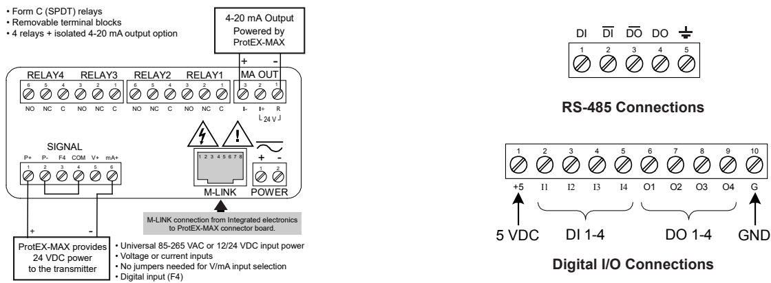
Connections for PD8-6000-6H7 & PD8-6000-7H7
