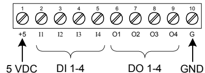
Digital I/O Connections
