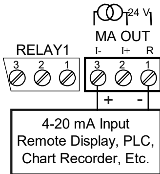
4-20 mA Output Powered by PD8-6001
