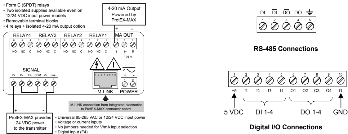
Connections for PD8-6001-6H7 & PD8-6001-7H7
