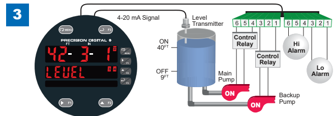
If the backup pump is not able to keep up, and the level reaches 40 FT , relay #4 transfers and starts the main pump as well.
