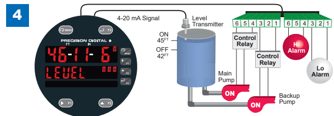
Relay #2 trips the High Level Alarm at 45 FT and resets at 42 FT .
