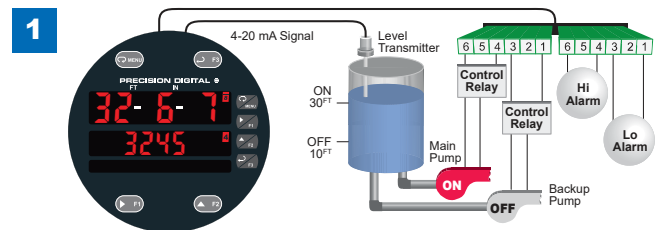
Relay #4 turns the main pump on at 30 FT and turns it off at 10 FT .
