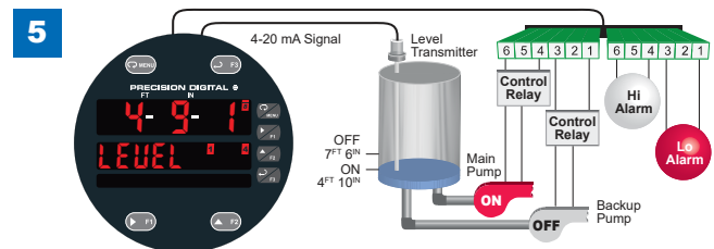
Relay #1 trips the Low Level Alarm at 4 FT 10 IN and resets at 7 FT 6 IN .
