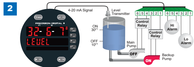
With the Pump Alternation feature activated, the next time the level reaches 30 FT , relay #3 transfers and starts the backup pump.
